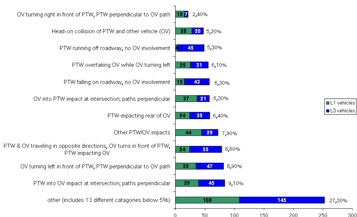
Figure 3.4: PTW accident configuration by legal category
