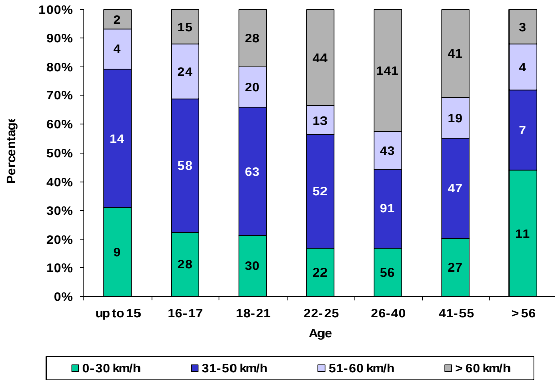
Figure 7.6: PTW travelling speed by PTW rider age
